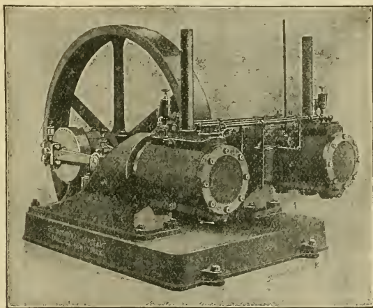
INGERSOLL-SERGEANT DUPLEX STEAM-DRIVEN AIR COMPRESSOR.
